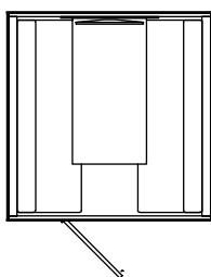
MEETING POD LARGE with integrated sofa's and low table. Sofa 1600mm x 665mm x 824mm
